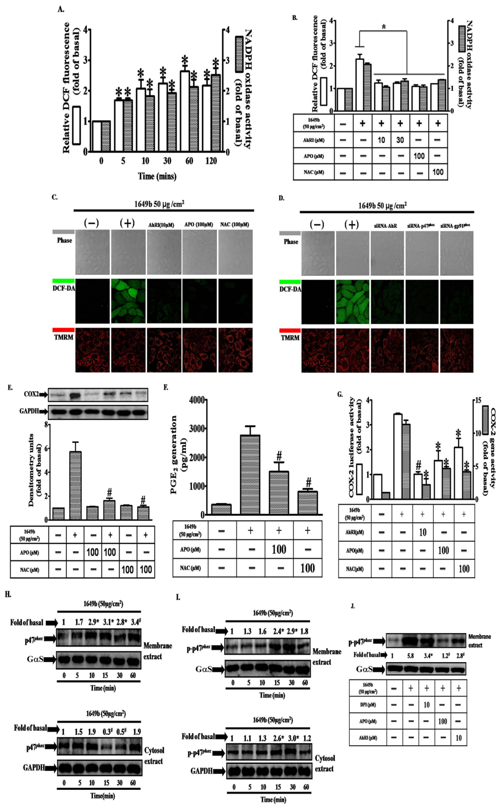
Figure 3. PMs induce NADPH oxidase activation, generation of reactive oxygen species (ROS) and p47 phox translocation in HaCaT cells. (A) Cells were exposed to PMs (50 µg/cm 2 ) for the indicated times (0, 5', 10', 30', 1 h and 2 h). (B) Cells were pre-incubated with AhRI (10 and 30 µM), APO (100 µM) or NAC (100 µM) for 1 h and then exposed to PMs (50 µg/cm 2 ) for 24 h. Effects of PMs and antioxidants on ROS generation (open bars) and NADPH oxidase activity (shaded bars) were measured using DCF-DA fluorescence and lucigenin chemiluminescence as described in “Materials and methods” (n = 3 in each group; *P < 0.05 compared with vehicle), respectively. (C,D) Cells were transfected with siRNAs of the aryl hydrocarbon receptor
