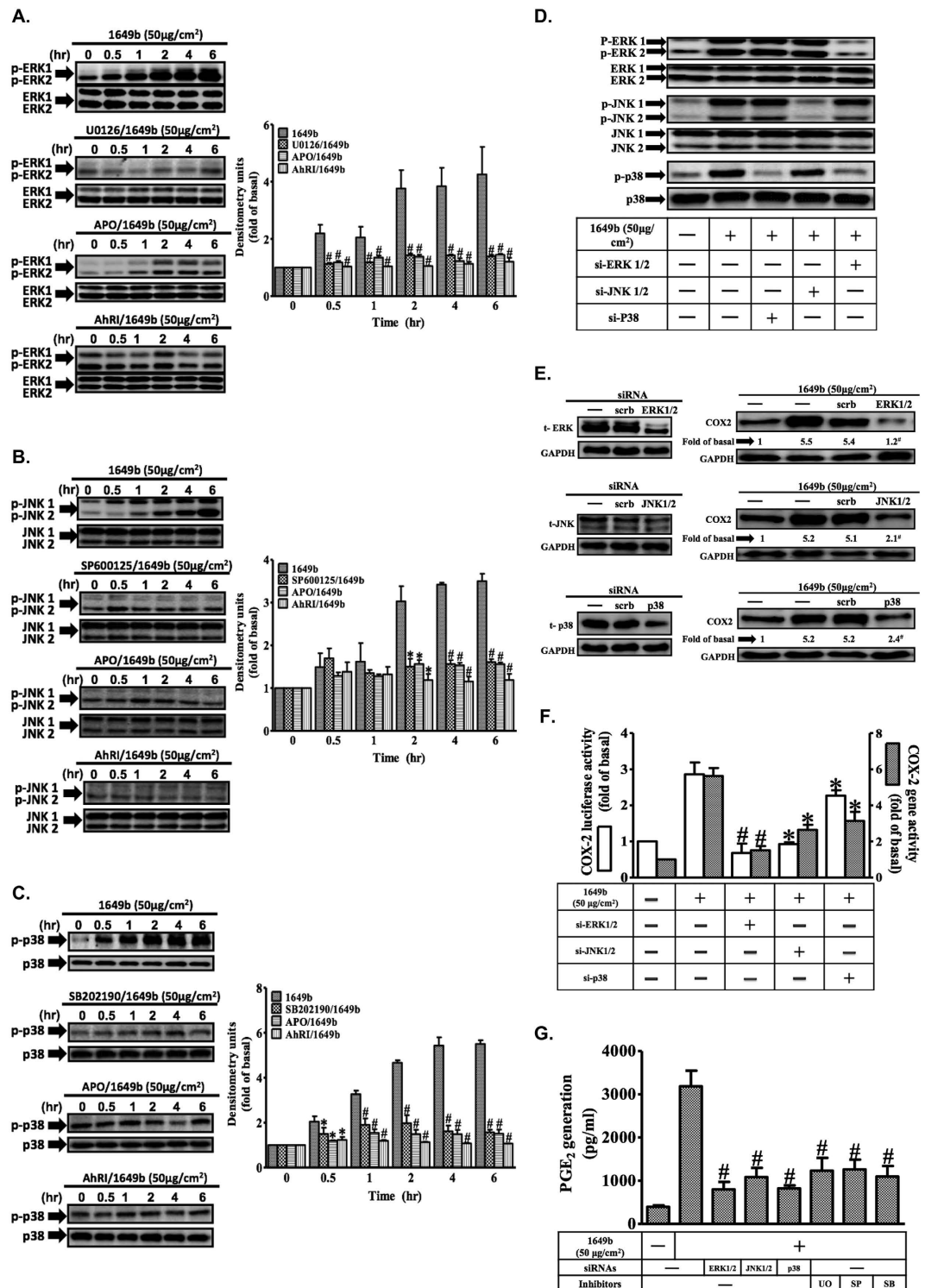
Figure 4. Reactive oxygen species (ROS)-dependent MAPK activation is involved in PMs-induced up-regulation of COX2 expression in HaCaT cells. Cells were pre-incubated with AhRI (10 µM), APO (100 µM), U0126 (10 µM), SB202190 (10 µM), SP600125 (10 µM) or DPI (10 µM) for 1 h and then exposed to PMs (50 µg/cm 2 ) for the indicated times (0, 30', 1 h, 2 h, 4 h and 6 h). (A–C) Effects of MAPK inhibitors and antioxidants on phosphorylation of p-ERK1/2 (A) p-JNK1/2 (B) and p-p38 (C) . Total levels of each kinase were used as loading controls. Effects of siRNAs or inhibitors of ERK1/2, JNK1/2 and p38 on the phosphorylation of MAPKs (D) COX2 protein expression (E) COX2 gene expression (F) and prostaglandin E2 (PGE2) production (G) . To assess gene expression (F) , cells were co-transfected with a COX2 reporter gene and following addition of siRNAs, exposed to PMs for 4 h (for promoter activity evaluations; open bars) or 6 h (for evaluations of mRNA levels; shaded bars). Representative results from three separate experiments are shown. * P < 0.05, # P < 0.01, compared with cells exposed to PM alone.
