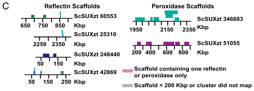
Fig. 4. Independent tandem gene cluster formation in squid and octopus and the origin of light organ-specific gene expression. Phylogenetic trees highlight highly specific expansion patterns that correlate with general shared expression between the light organ and the eyes for reflectins (A) or the appearance of the light organ-specific expression pattern for heme peroxidases (B). Heat maps indicate relative normalized expression levels for each tissue (Z scores). Scale bar underneath phylogenetic trees indicates amino acid substitutions per site. Color of the nodes (A and B) identifies genomically colocalized genes (shown in C). Those genes are clustered in tandem on several scaffolds with positions and gene identifiers labeled. (C) Tandem clusters of reflectin and peroxidase genes in the E. scolopes genome. Scaffold ID and approximate location (kbp) is shown for each gene (represented by rectangle). Colors correspond to the sequences on the trees in A for reflectins and (B) for peroxidases.
