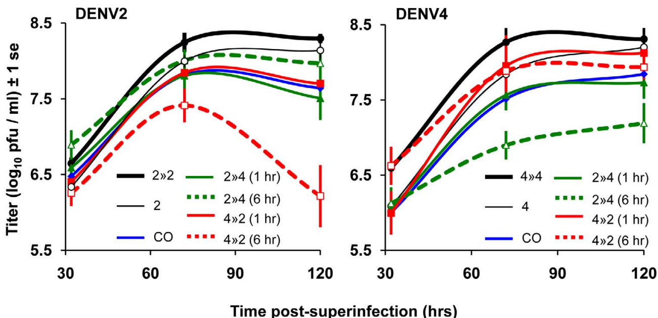
Figure 1 Titers over time. Mean titers are plotted against the superinfection interval for DENV2 (left) and DENV4 (right). Bars indicate standard errors of the mean (N = 4). Single-serotype infections are in black, mixed-serotype infection treatments are: coinfections (blue), superinfection of DENV4 after DENV2 (green), and superinfection of DENV2 after DENV4 (red). Treatment abbreviations correspond to the treatments described in Table 1.
