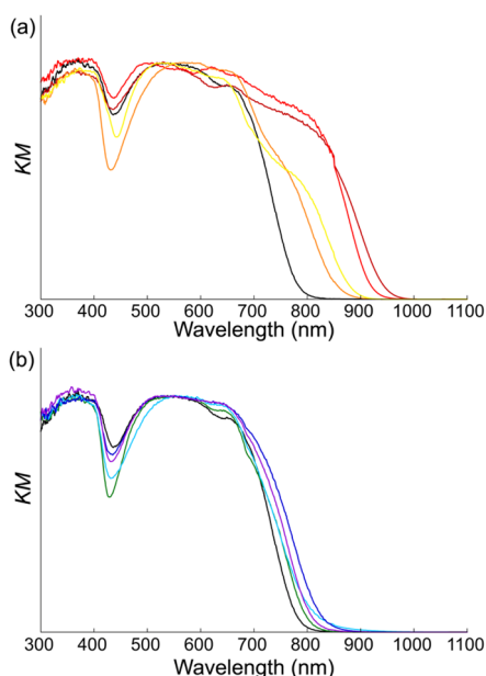
Fig. 7 Comparison of diffuse reflectance spectra of Cn^{2+} \cdot 2CMI^- (a) n = 1\text{--}4 and (b) n = 5\text{--}8 with Na^+CMI^- . Spectra line colour code: black, dark red, red, orange, yellow, green, light blue, blue and purple refer to Na^+CMI^- , C1^{2+} \cdot 2CMI^- , C2^{2+} \cdot 2CMI^- , C3^{2+} \cdot 2CMI^- , C4^{2+} \cdot 2CMI^- , C5^{2+} \cdot 2CMI^- , C6^{2+} \cdot 2CMI^- , C7^{2+} \cdot 2CMI^- and C8^{2+} \cdot 2CMI^- , respectively.
