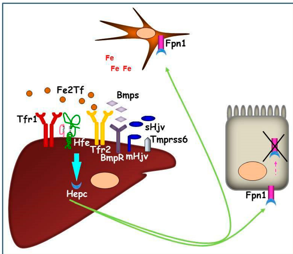
Figure 2. Graphic representation of the hepatic Hepc pathway in conditions of systemic iron increase. The iron signaling proteins (Fe 2 Tf and Bmps) interact with iron sensors (Tfr1, Hfe, Tfr2, BmpRs) and their co-activator (mHjv) to promote Hepc production. Hepc, secreted by hepatocytes, is transported in plasma and binds iron exporter Fpn1 on duodenal and reticuloendothelial cell surfaces causing its internalization and intracellular degradation. As a consequence, iron remains entrapped in these cells, systemically reducing the metal availability.
