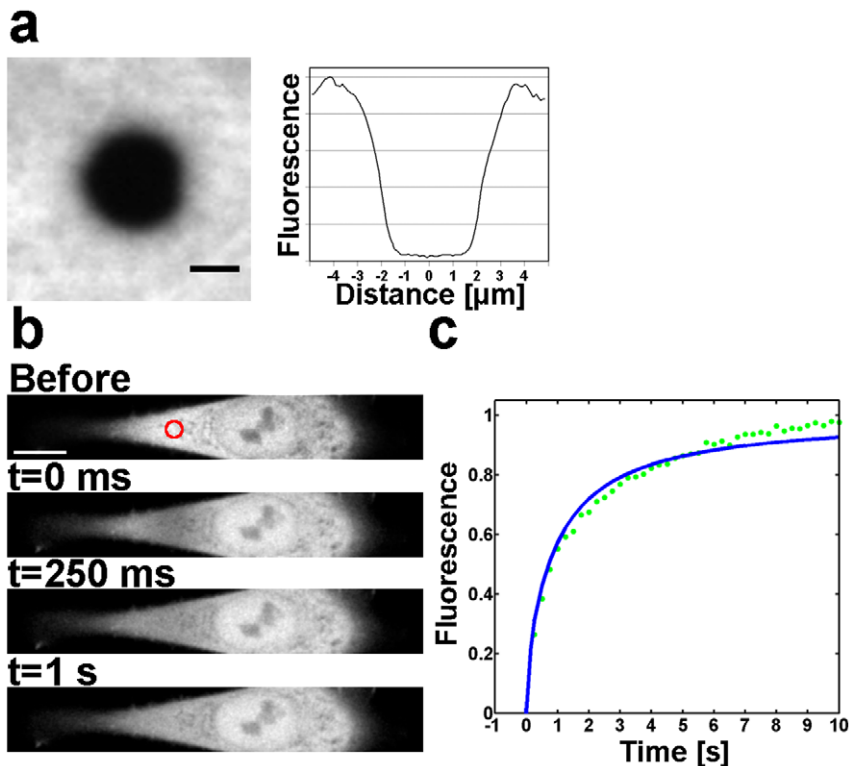
Figure 1. FRAP experiment in an NLFK cell stably expressing EYFP. (a) The average ( n=10 ) bleach profile measured on fixed cells expressing EYFP. Scale bar 2 \mu\text{m} . (b) Fluorescence distribution before the bleach pulse and the position of the circular bleach area (diameter 20 pixels, FWHM 3.7 \mu\text{m} ). Subsequent images show the fluorescence distribution immediately ( t=0 ms), and 250 ms and 1 s after the bleach pulse. Scale bar 10 \mu\text{m} . (c) The measured recovery curve (Axelrod normalization) and a fit by the free-diffusion model of Soumpasis. doi:10.1371/journal.pone.0022962.g001
