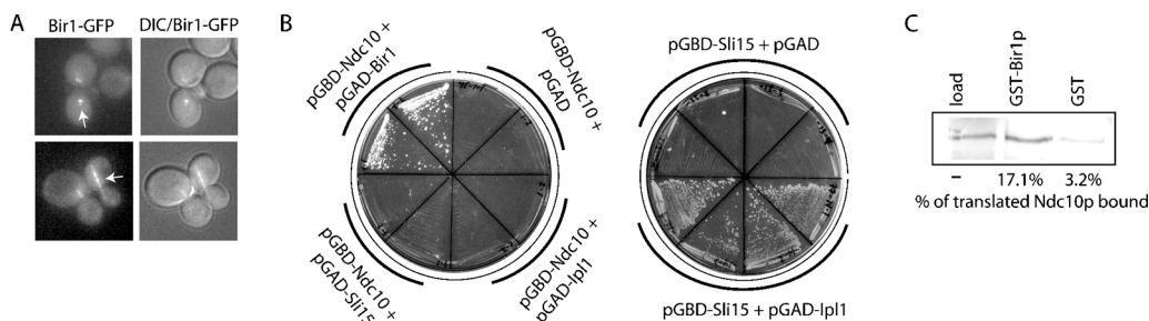
Figure 7. Bir1p localizes to inter-polar microtubules and interacts with Ndc10p. (A) Bir1-GFP was imaged in premetaphase cells (top, arrow) and in anaphase cells (bottom, arrow); fluorescence and DIC images were recorded. (B) The indicated bait and prey yeast two-hybrid vectors were plated on HIS selection; growth indicates an interaction. (C) Ndc10p was translated in vitro in the presence of ^{35} S-methionine. The translated protein was incubated with GST-Bir1p or GST and the fraction of the Ndc10p bound to the beads was calculated.
