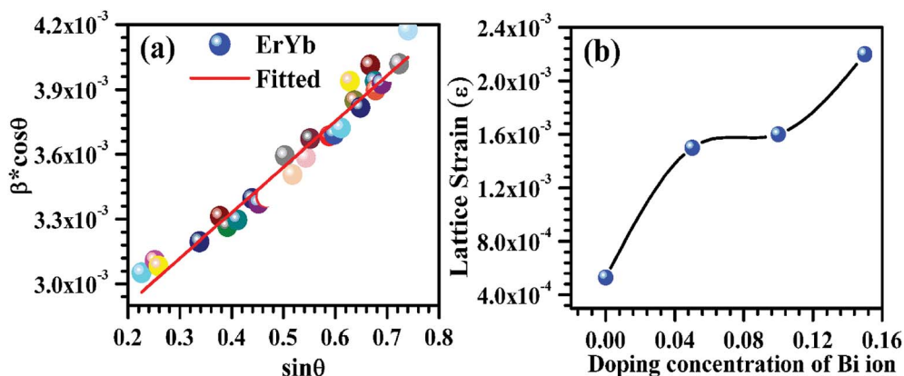
Fig. 5 (a) A Williamson–Hall plot of the \text{Er}^{3+}/\text{Yb}^{3+} co-doped \text{La}_2\text{O}_3 nano-phosphor sample and (b) a variation in lattice strain as a function of different concentrations of \text{Bi}^{3+} ions ( i.e. 0, 5, 10 and 15 mol%).
