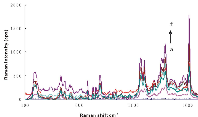
Figure 4. SERS spectrum of AuNP B -HAuCl 4 -H 2 O 2 -VBB system. (a) 4.48 \mu\text{mol/L} HAuCl 4 +0.67 mmol/L HCl+3.33 mmol/L H 2 O 2 +1.3 \mu\text{mol/L} VBB (b) a+19 ng/mL AuNP B ; (c) a+38 ng/mL AuNP B ; (d) a+95 ng/mL AuNP B ; (e) a+190 ng/mL AuNP B ; (f) a+285 ng/mL AuNP B .
