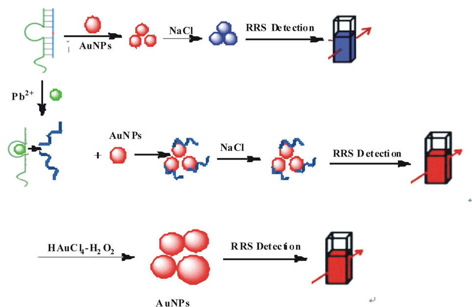
Figure 10. Principle of aptamer nanogold catalytic detection of \text{Pb}^{2+} with RRS effects.
