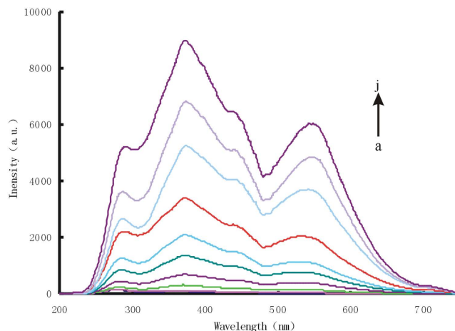
Figure 1. RRS spectrum of AuNP c -HAuCl 4 -H 2 O 2 system. (a) 4.48 μmol/L HAuCl 4 +0.67 mmol/L HCl+3.33 mmol/L H 2 O 2 (b) a+1.9 ng/mL AuNP c ; (c) a+3.8 ng/mL AuNP c ; (d) a+7.6 ng/mL AuNP c ; (e) a+19 ng/mL AuNP c ; (f) a+34.2 ng/mL AuNP c ; (g) a+47 ng/mL AuNP c ; (h) a+85.5 ng/mL AuNP c ; (i) a+133 ng/mL AuNP c ; (j) a+161.5 ng/mL AuNP c .
