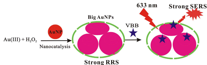
Figure 9. Small AuNPs catalyze the \text{H}_2\text{O}_2 reduction of \text{HAuCl}_4 to big AuNPs with SERS and RRS effects.
