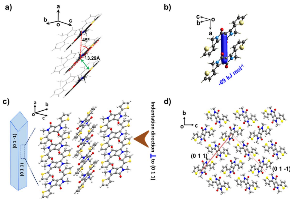
Fig. 2 Crystal packing of DPP-diMe crystals. (a) \pi -Stacked columns, extended along the crystal growth direction, with a slip-stack angle of 45^\circ and interplanar distance of 3.298 \text{ \AA} and (b) the corresponding pairwise total interaction energy, E_{\text{total}} = -69 \text{ kJ mol}^{-1} (calculated from the CIF obtained from SCXRD). (c and d) Packing patterns viewed along different directions.
