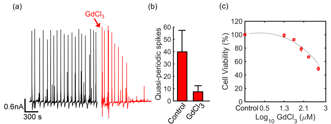
Figure 6. Selective blocking of Ca^{2+} stretch-activated channels. (a) Diatoms were kept in dark for more than 2 day/night cycles. The black trace of the current recording depicts the current fluctuations at the start of the experiment. The red trace is obtained after adding the inhibitor GdCl_3 to the culture medium up to a concentration of 100 \mu M . (b) Data quantification recorded over 3 experiments. Current spikes were counted 45 minutes before, called control, and after adding the inhibitor, called GdCl_3 . (c) Cell viability in percentage upon exposure for 24 hours to different concentrations of GdCl_3 ; at 100 \mu M there is no impact on cell viability.
