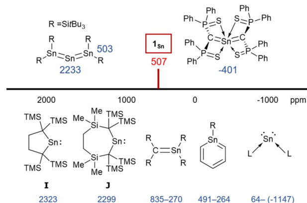
Fig. 4 ^{119}\text{Sn} NMR chemical shifts of \mathbf{1}_{\text{Sn}} and related compounds.
