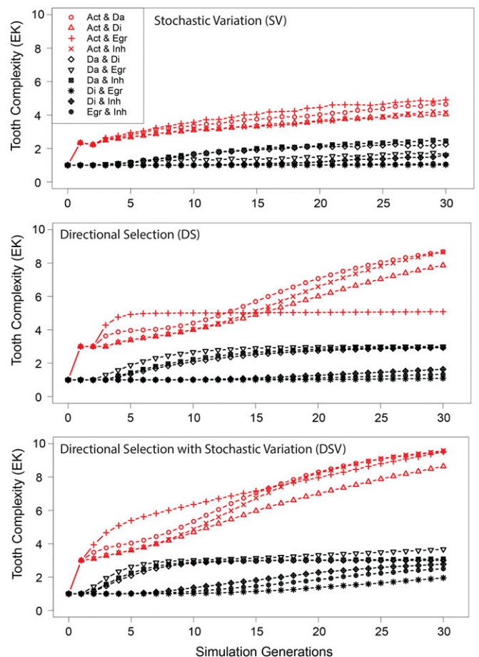
Fig. 4. Simulations of tooth complexity evolution across 10 developmental landscapes under different models of evolution. Lines are means of 10,000 evolutionary simulations, each run for a maximum of 30 generations. Red denotes landscapes where activation (Act) was varied. Evolutionary models were the following: 1) stochastic variation (SV), 2) directional selection (DS) for enamel knot (EK) number, and 3) directional selection with stochastic variation (DSV). The parameter abbreviations are the following: activator self-regulation (Act), activator diffusion rate (Da), inhibitor diffusion rate (Di), epithelial growth rate (Egr), and strength of inhibition (Inh).
