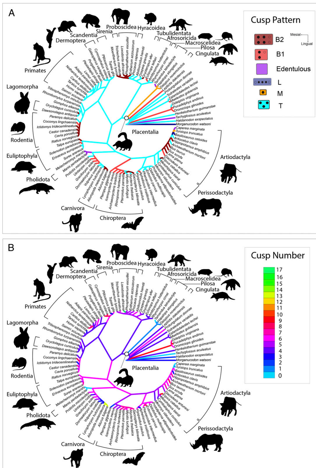
Fig. 6. Ancestral state reconstruction of tooth cusp pattern (A) and tooth cusp number (B) across a phylogeny of 93 species of fossil and extant placentals and closely related taxa. All data collected from the upper second molar. Tree modified after the phylogeny of ref. 21. (Clockwise from Top Left) images credit: Wikimedia Commons/Nina Holopainen/Stavenn/Joey Makalintal/birdphotos/PD-USGov/Thomas Hardwicke.
