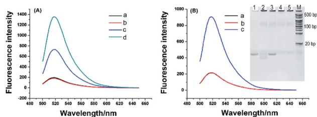
Fig. 2 (A) Fluorescence spectra of (a) 1 μM RNA probe, (b) reaction products with 1 μM RNA probe and 1 μM TS primer, (c) reaction products with 1 nM RNA probe and 1 nM TEP, and (d) reaction products with 1 μM RNA probe and 1 nM TEP. (B) Fluorescence spectra of reaction products with (a) lysis buffer, (b) heat-inactivated telomerase extracts, (c) telomerase extracts equivalent to 800 HeLa cells. Inset: non-denaturing PAGE analysis of the telomerase activity. Lane M: double strand DNA ladder, lane 1: TS primer (100 nM), lane 2: reaction products with telomerase extracts, lane 3: reaction products with heat-inactivated telomerase extracts, lane 4: telomerase extracts, lane 5: heat-inactivated telomerase extracts equivalent to 800 HeLa cells.
