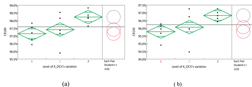
Fig. 11 One-way ANOVA diagram of CR_i versus the CV_{K\_OCV} level, based on the modeling and validation data set: (a) diagram of CR_{100} versus the CV_{K\_OCV} level; and (b) diagram of CR_{150} versus the CV_{K\_OCV} level.
