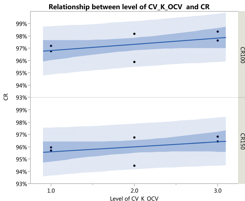
Fig. 10 Relationship between the level of CV_{K\_OCV} and CR. The line is the linear fit of the data, while the dark and light blue bands correspond to the confidence interval and the prediction interval of the data, respectively, based on the fitting.
