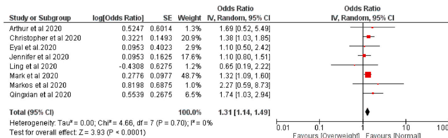
Fig. 5. Forest plot illustrating the Random effect model of the association between obesity and COVID-19 severity.
