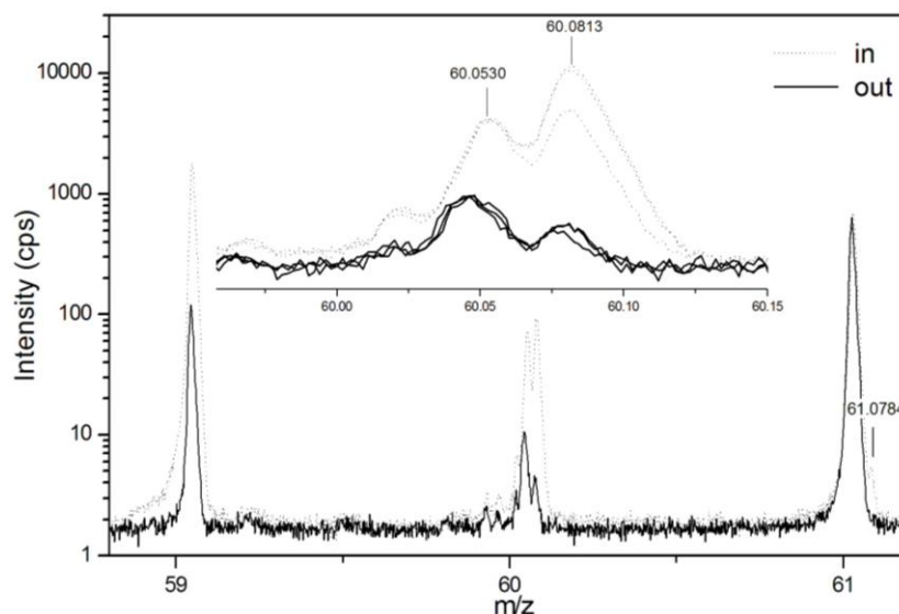
Figure 6. Excerpt of the PTR-TOF-MS spectra of six samples collected upstream (dotted lines) and downstream (continuous lines) a biofilter. The upper panel is a detail of the peak at m/z = 60 . Numbers indicate the expected exact mass of protonated monosubstituted acetone isotope (60.053) and of protonated trimethylamine (60.0813). At mass 61.0784 the mono substituted isotope of trimethylamine is also indicated. Reprinted from [129], with permission from the copyright holders, IWA Publishing.
