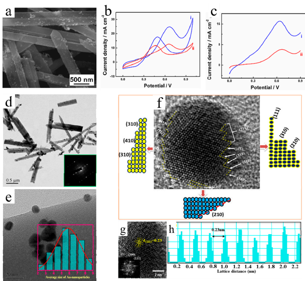
Figure 5. (a) FESEM image of the prepared Pt/ \text{MoO}_3 nanocatalysts; (b) CVs of the (i) Pt/ \text{MoO}_3 and Pt/C (ii) catalysts in 0.5 M of \text{H}_2\text{SO}_4 containing 1.0 M of \text{CH}_3\text{OH} ; (c) LSVs of the (i) Pt/ \text{MoO}_3 and Pt/C (ii) catalysts in 0.5 M of \text{H}_2\text{SO}_4 containing 1.0 M of \text{CH}_3\text{OH} [86]. Reprinted with permission from [86]. Copyright 2015 Elsevier B.V. (d) TEM image of Au/ \text{MoO}_3 (inset: corresponding SAED pattern); (e) HRTEM image of Au/ \text{MoO}_3 (inset: the average size of Au nanocrystals calculated from histograms); (f) Typical HRTEM lattice image of high index surfaces Au nanocrystals; (g) HRTEM image shows the majority of lattice plane (111) facet of Au nanocrystals, the inset in (g) indicates FFT pattern of Au nanocrystals enclosed with (111) and (200) plane; (h) IFFT profile of Au nanocrystals lattice distance analysis [91]. Reprinted with permission from [91]. Copyright 2017 Elsevier Ltd.
