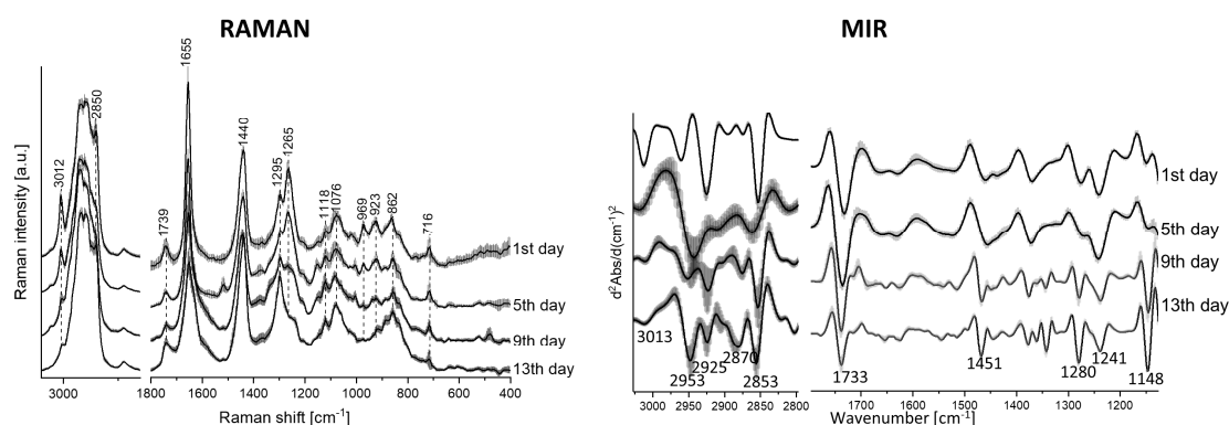
Figure 8. Averaged Raman (left) and second derivative MIR (right) spectra with standard deviation ( \pm SD) for lipids of medaka fish eggs collected on the 1st, 5th, 9th, and 13th day after fertilization.
