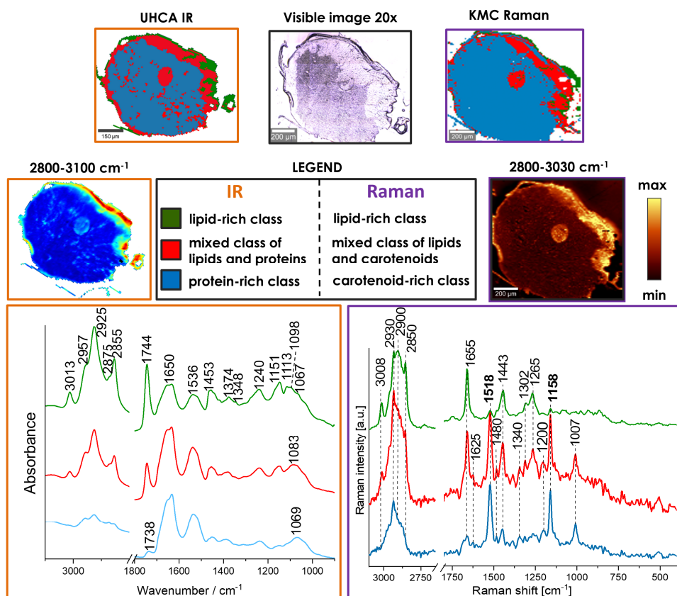
Figure 7. MIR (left) and Raman (right) images with their cluster analysis of a cross-section of a medaka fish egg collected on day 1 after fertilization; MIR and Raman spectra are mean spectra calculated in cluster analysis (the colors of spectra correspond to the colors of classes).
