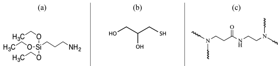
Fig. 1 Chemical structure of (a) 3-(aminopropyl)-triethoxysilane, (b) 1-thioglycerol and (c) repeating unit of poly-(amidoamine)-(NH 2 ) 4 dendrimer.
