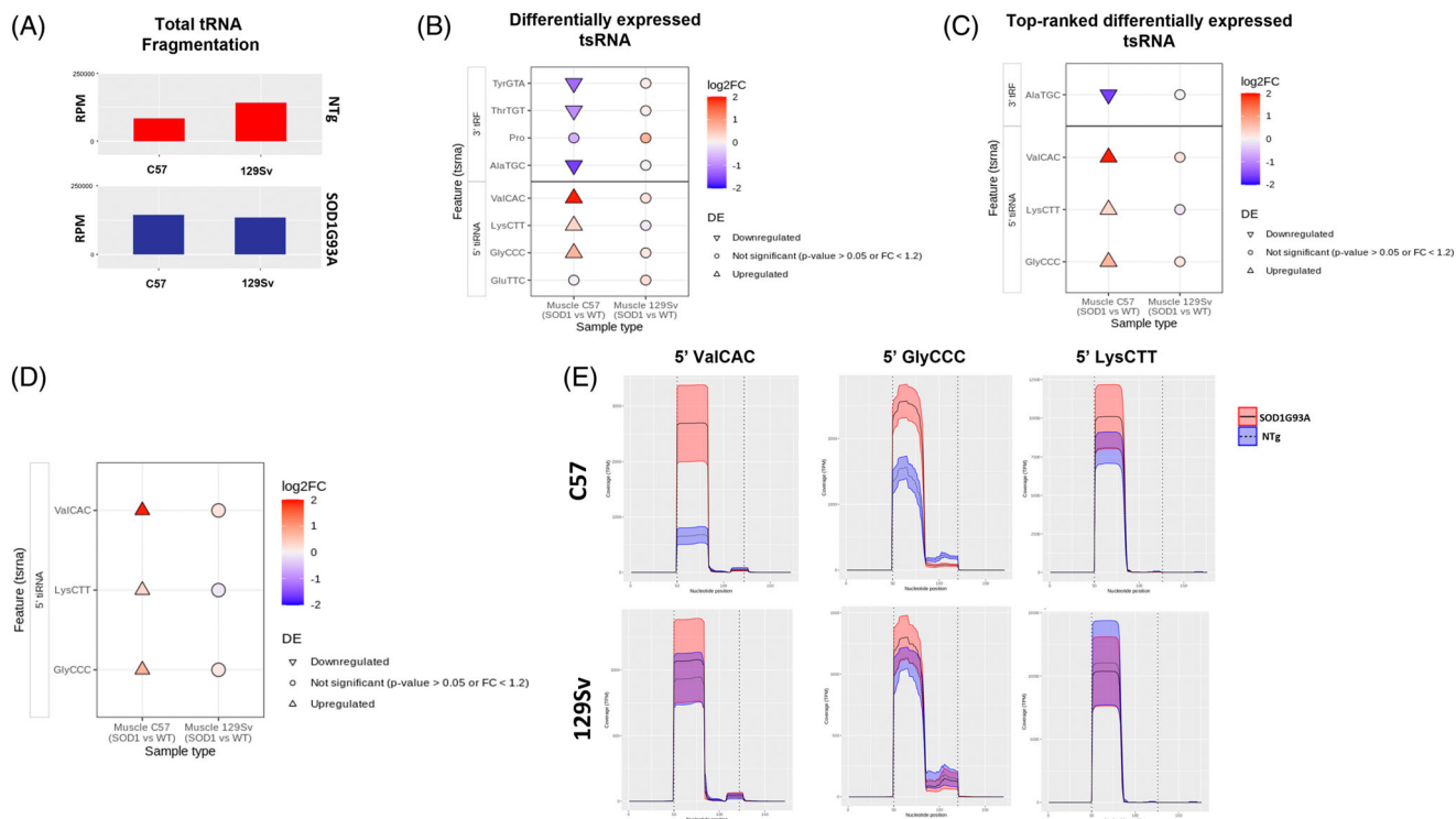
FIGURE 3 TsRNAs identified in RNA sequencing data from muscle tissue samples. (A) Normalised tRNA read counts identified in the NTg and SOD1G93A in C57 and 129Sv genetic backgrounds. (B) Summary of differentially expressed tsRNAs from the SOD1G93A versus NTg comparison in the C57 and 129Sv genetic background. The shape represents the regulation; upward facing arrow for upregulated, downward facing arrow for downregulated and a circle for not significant and the colour indicates the log2FC. (C) Summary of top differentially expressed tsRNAs with mean TPM greater than 100 from the SOD1G93A versus NTg comparison in the C57 and 129Sv genetic background. (D) Summary of top differentially expressed tsRNAs from the SOD1G93A versus NTg comparison in the C57 and 129Sv genetic background. (E) Coverage plots of 5' ValCAC, 5' GlyCCC, 5' LysCTT tsRNAs identified as top differentially expressed tsRNAs. The x-axis represents the nucleotide position and the y-axis represents the coverage in TPM. The two vertical dotted lines enclose the main tRNA segment of 70 bp, with an additional 50 bp included both upstream and downstream. The dotted line illustrates the mean coverage for NTg samples, while the solid line represents the mean coverage for the SOD1G93A condition, with the shaded areas indicating the standard deviation for both conditions.
