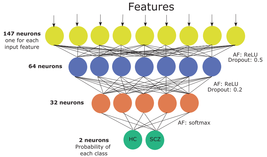
FIGURE 3 Scheme of the MLP composed of four layers: input layer, two hidden layers and the output layer. AF, activation function.
