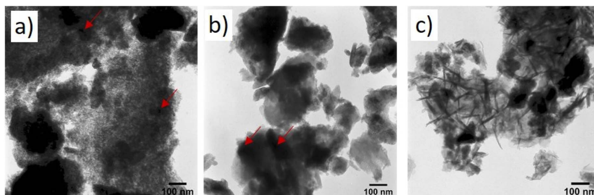
Fig. 13 TEM images of Al 2 O 3 /SrCO 3 sol-gel incorporated with Pt after annealing at 500 °C, showing molar ratios of: (a) Sr : 0.1 Pt, (b) Sr : 0.25 Pt, and (c) Sr : 0.5 Pt. 51
