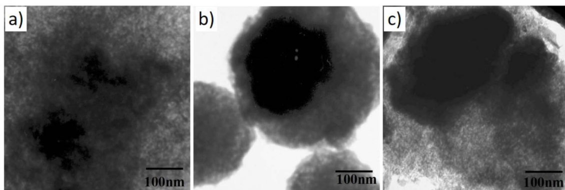
Fig. 12 TEM images of Al 2 O 3 /SrCO 3 xerogels annealed at 500 °C, illustrating different Sr/Al molar ratios: (a) 0.1, (b) 0.5, and (c) 1.0. 51
