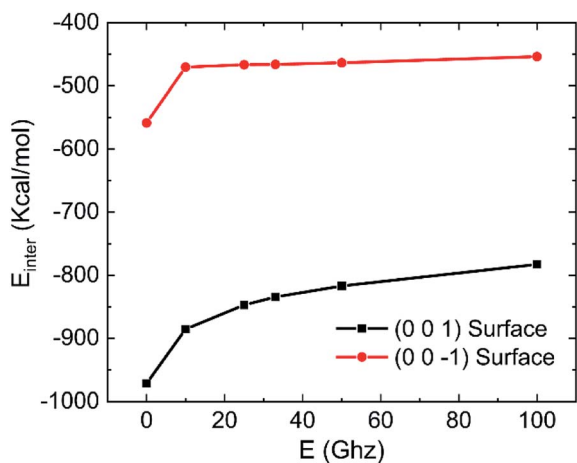
Fig. 18 Effects of frequency on the interaction energy between water and kaolinite ( 0.25 \text{ V \AA}^{-1} , 333.15 K).
