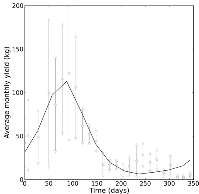
Figure 2. Model output and data from the study area (zoom on year 10). The solid black curve corresponds to the model output, the gray dots to the average monthly yields observed in the six plots of the study area. The grey bars around these dots correspond to the average values \pm standard deviation. doi:10.1371/journal.pone.0080352.g002
