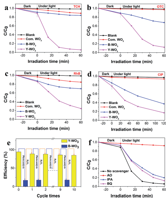
Fig. 4 The photocatalytic efficiencies of TCH, OTC, RhB and CIP over Y-WO 3 and B-WO 3 under visible light irradiation (a–d); the stability and reusability of the as-synthesized samples (e); active species trapping experiments of Y-WO 3 under visible light irradiation (f).
