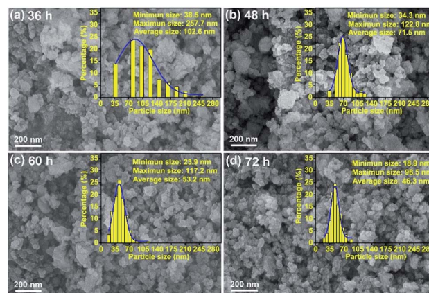
Fig. 2 SEM images of HEO nanoparticles with ball-milled time of: (a) 36 h; (b) 48 h; (c) 60 h; (d) 72 h. The inserted graphs show the corresponding size distribution histograms and the calculated average particle size of HEO nanoparticles.
