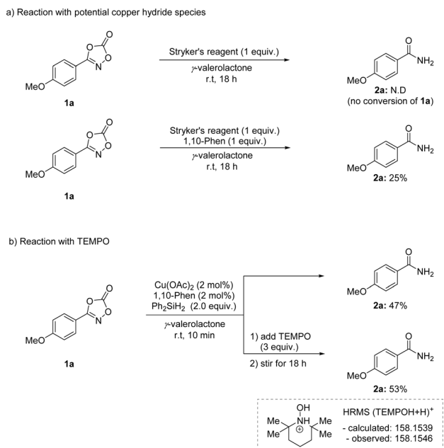
Scheme 6 Mechanistic studies.
