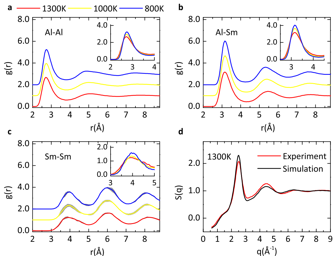
Figure 4. Validation of \text{Al}_{450}\text{Sm}_{50} AIMD simulations. (a–c) The PCF averaged over three AIMD \text{Al}_{450}\text{Sm}_{50} samples for Al–Al, Al–Sm and Sm–Sm, respectively. The grey error band is generated by sweeping the error bar over all positions. The curves of different temperatures are shifted vertically for clarity. The inserts zoom in the first peak which is enhanced during the cooling process. (d) The structure factor obtained from AIMD simulations and experiments.
