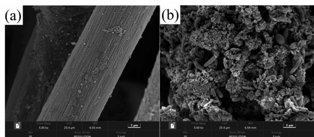
Fig. 3 SEM image of (a) raw graphite felt and (b) anode biofilm of the DLCW-MFC.
