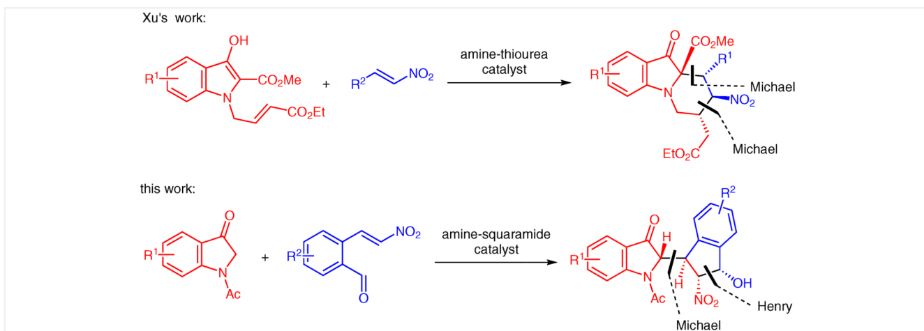
Scheme 1. Indolin-3-one in organocatalytic asymmetric domino reactions
