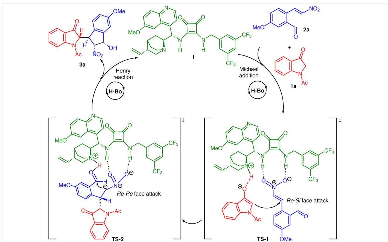
Scheme 2. Proposed reaction mechanism
