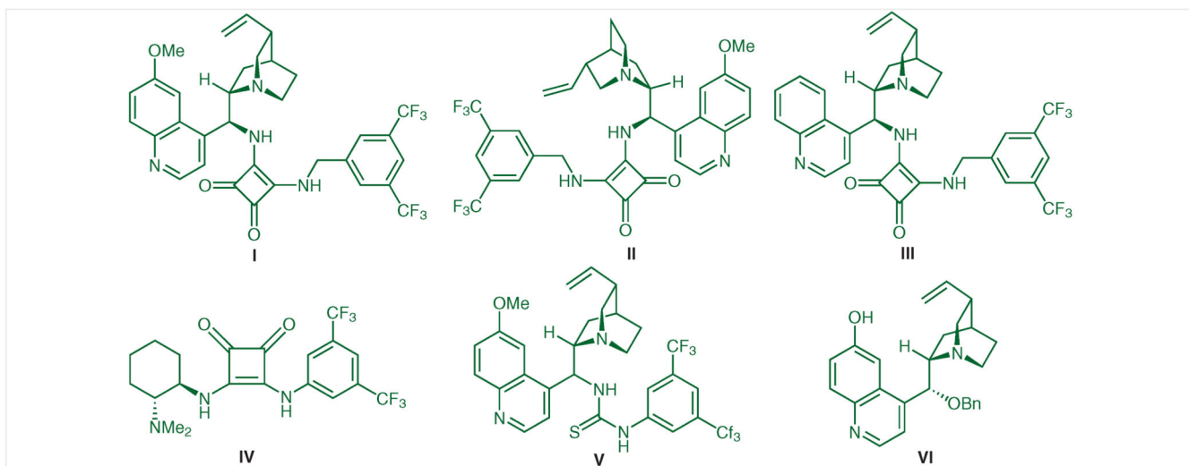
Figure 2. Organocatalysts used
