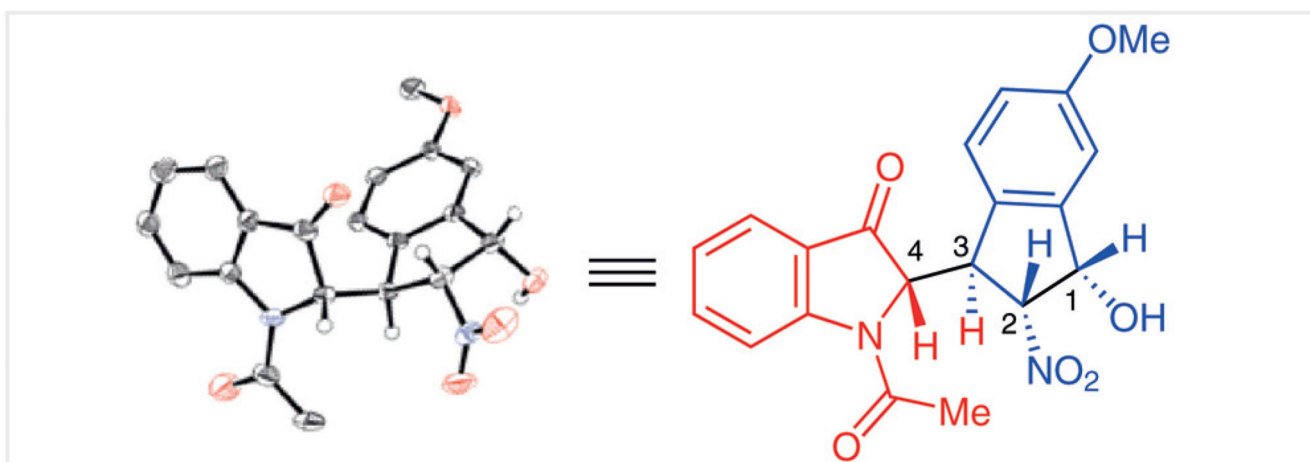
Figure 3. Determination of the absolute configuration of 3a by the X-ray crystal structure analysis
