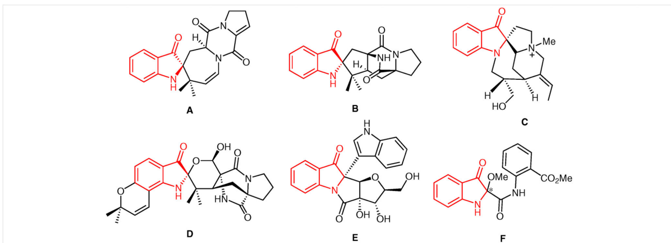
Figure 1. Representative examples of natural products bearing the indolin-3-one unit
