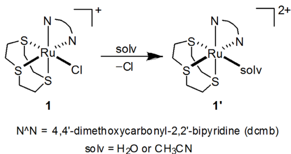
Figure 1 | Chemical structure of ruthenium(II) complexes 1' , formed from the in situ hydrolysis of complex 1 .
