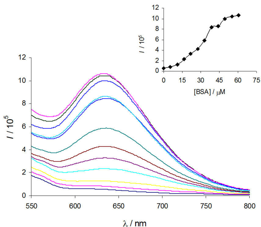
Figure 3 | Phosphorescence emission spectra of 1' (50 μM) in H 2 O with increasing concentration of [BSA]/[1'] (0–1.2) at 20°C. Inset: phosphorescence emission intensity at 630 nm vs. BSA concentration.
