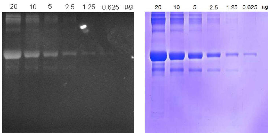
Figure 4 | Left: Emissive SDS-PAGE analysis of BSA with complex 1' (2.6 mg/20 mL) as the detecting agent (staining time: 30 min); Right: Control SDS-PAGE analysis of BSA with Coomassie Brilliant Blue staining (staining: 60 min; destaining: 24–48 h).
