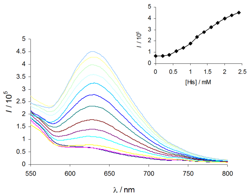
Figure 2 | Phosphorescence emission spectra of 1' (50 μM) in 5% CH 3 CN/95% H 2 O with increasing concentration of [His]/[1'] (0–48) at 20°C. Inset: phosphorescence emission intensity at 630 nm vs. His concentration.
