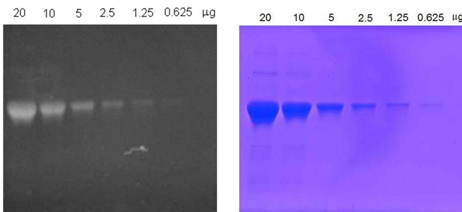
Figure 5 | Left: Emissive SDS-PAGE analysis of 6xHis-tagged NF-κB p50 with complex 1' (2.3 mg/20 mL) as the detecting agent (staining time: 30 min); Right: Control SDS-PAGE analysis of BSA with Coomassie Brilliant Blue staining (staining: 60 min; destaining: 24–48 h).
