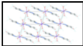
Fig. 2. View of the three-dimensional network of the title compound, built by hydrogen bonds (dashed lines).
