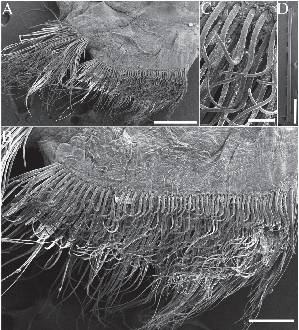
Figure 5. SEM pictures of Phyllo fimbriata (Moore, 1903) A anterior thoracic chaetiger, anterior view B same, detail, showing arrangement of neurochaeta C same, detail, showing neurochaetae D modified spines. Scale bars: 5 mm ( A, D ); 200 µm ( B ); 50 µm ( C, D ).
