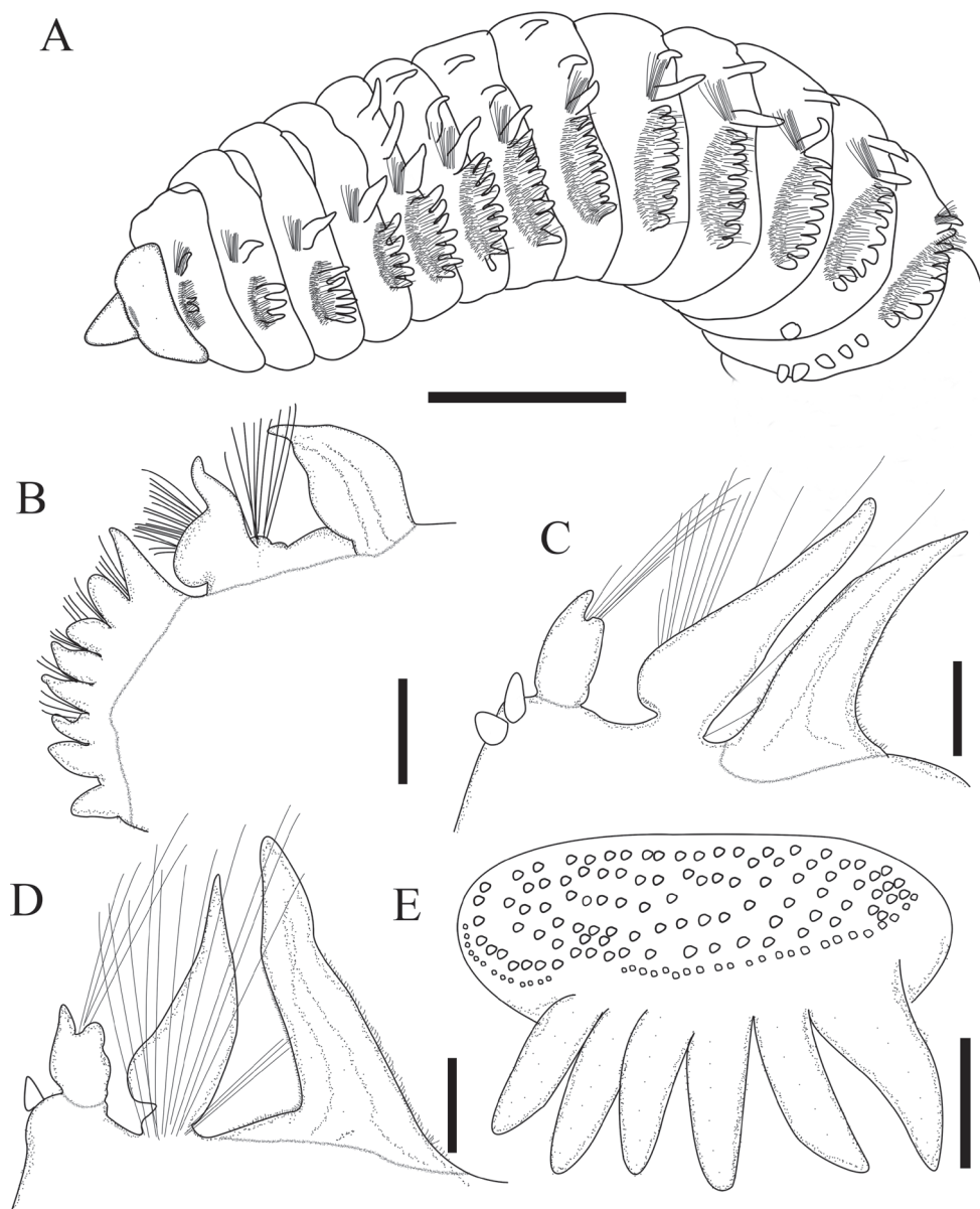
Figure 2. Phylo heterochaetus sp. nov. A anterior body in lateral view B parapodium of chaetiger 7 C parapodium of anterior abdominal chaetiger D parapodium of chaetiger 62 E diagram showing arrangement of anterior thoracic neurochaetae. Scale bars: 2 mm ( A ); 400 \mu m ( B–D ); 200 \mu m ( E ).
