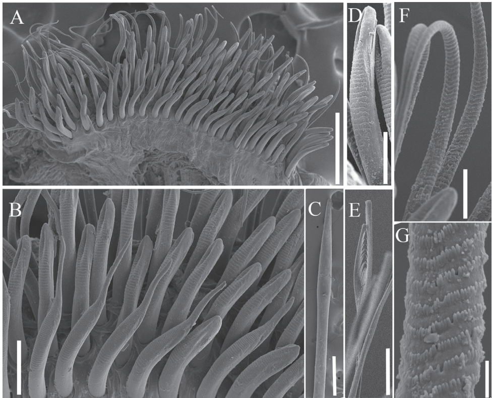
Figure 3. SEM pictures of Phyllo heterochaetus sp. nov. A neurochaetae of thorax B uncini and subuluncini C modified spines D uncini of last rows of thoracic neuropodia E furcate chaeta F, G crenulate capillaries. Scale bars: 250 \mu\text{m} ( C ); 200 \mu\text{m} ( A, E, F ); 50 \mu\text{m} ( B ); 30 \mu\text{m} ( G ); 10 \mu\text{m} ( D ).
