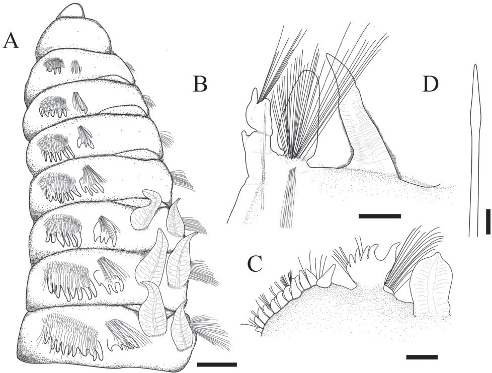
Figure 4. Phylo fimbriata (Moore, 1903) A anterior end, left lateral view B parapodium of abdominal chaetigers; C parapodium of thoracic chaetigers D modified spine from posterior thoracic chaetiger. Scale bars: 1 mm ( A ); 500 \mu m ( B–D ).
