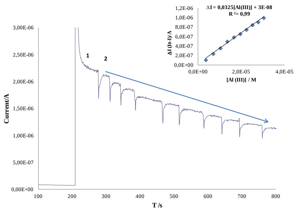
Figure 3. Typical amperometric recording for an acetylthiocholine iodide concentration (1) 2.4 \times 10^{-4} M and consecutive additions of aliquots of Al(III) solution into the cell to give an overall concentration of: (2) 3.6 \times 10^{-6} , (3) 7.0 \times 10^{-6} , (4) 1.0 \times 10^{-5} , (5) 1.3 \times 10^{-5} , (6) 1.6 \times 10^{-5} , (7) 1.9 \times 10^{-5} , (8) 2.2 \times 10^{-5} , (9) 2.5 \times 10^{-5} , (10) 2.8 \times 10^{-5} , (11) 3.0 \times 10^{-5} ; Britton-Robinson pH 7.8; Eap, + 0.8 V vs. Ag/AgCl screen-printed electrode.
