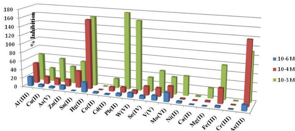
Figure 5. Inhibition percentage of inhibition current of ACh AuNPs/SPCE in presence of: Cu(II); As(V); As(III); Zn(II); Sn(II); Hg(II); Co(II); Cd(II); Pb(II); W(VI); Se(IV); V(V); Mo(VI); Ni(II); Ca(II); Mg(II); Fe(III); Cr(III); As(III) at 10 -6 M; [ATI] 0.12 \mu M; Eap, + 0.8 V vs. Ag/AgCl screen printed electrode; Britton-Robinson pH 7.8.
