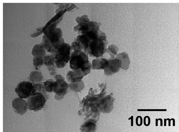
Fig. 6 TEM image of 7% Ni doped \text{Mn}_3\text{O}_4 NPs.
