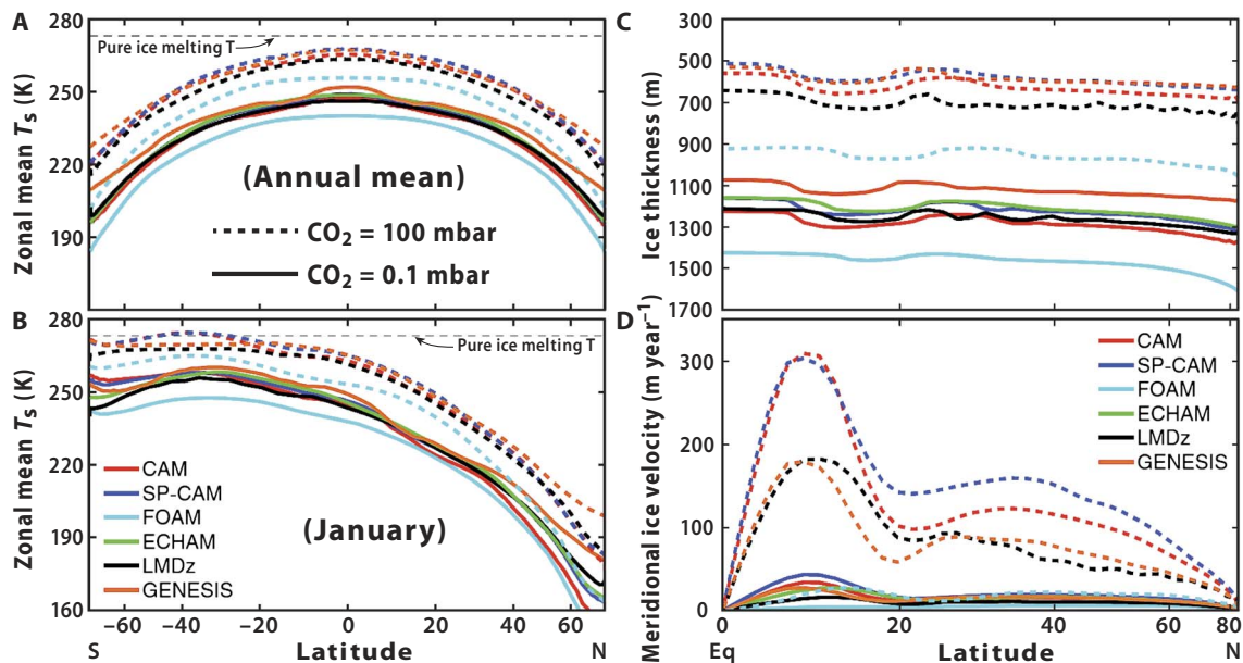
Fig. 8. Snowball Earth intermodel comparison (81). Colors assigned each GCM as indicated in (B). Solid lines, \text{CO}_2 = 0.1 mbar; dashed lines, \text{CO}_2 = 100 mbar. To isolate differences in atmospheric behavior among models, surface albedo was set to 0.6 everywhere, eliminating differences between ablative and snow-covered ice. Topography and the radiative effect of aerosols were set to zero, as were all greenhouse gases other than \text{CO}_2 and \text{H}_2\text{O} . The solar constant was set to 94% (present-day value; 1285 \text{ W m}^{-2} ), obliquity was set to 23.5^\circ , and eccentricity was set to zero. (A) Annual and zonal mean surface temperature. (B) January zonal mean surface temperature. (C) Sea-glacier thickness in meters (increasing downward to simulate depth below the ice surface). (D) Meridional (equatorward) ice velocity in meters per year. Models used are as follows: CAM (Community Atmosphere Model) (489), SP-CAM (Super-Parameterized Community Atmosphere Model) (490, 491), FOAM (Fast Ocean Atmosphere Model) (492), ECHAM (European Centre Hamburg Model) (493), LMDz (Laboratoire Météorologie Dynamique Zoom) (256), and GENESIS (Global Environmental and Ecological Simulation of Interactive Systems) (494, 495). FOAM produces surface temperatures substantially lower than those of other models and ice was accordingly thicker and slower. This is because FOAM is essentially a cloud-free model under Snowball conditions, accounting for its anomalous resistance to deglaciation at a geologically feasible \text{CO}_2 level (80, 82, 228).
