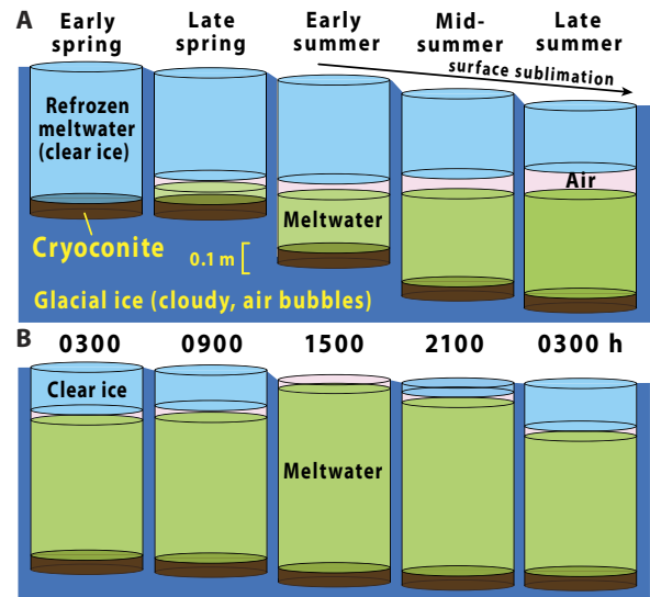
Fig. 14. Meltwater cycles in polar and low-latitude cryoconite holes. (A) Summer seasonal cycle of a cryoconite hole in the sublimation zone on Canada Glacier (Fig. 13B), Taylor Valley, Antarctica (279). In early summer, cryoconite melts to an equilibrium depth, after which it maintains constant depth relative to the sublimating surface. Air is evolved in the hole from melting of glacial ice containing bubbles of air and from photosynthetic O_2 production. Meltwater refreezes in winter and is covered by an ice cap in summer. Cryoconite is suffused with filamentous cyanobacteria and extracellular mucilaginous polysaccharides, and the holes are also inhabited by green algae, fungi, protists, and certain bilaterian animals—nematodes, rotifers, and tardigrades (282). (B) Postulated diurnal cycle (0000 hour) of a cryoconite hole on the low-latitude sublimation zone of a sea glacier on Snowball Earth. Relatively high CO_2 allows the nocturnal ice cap to melt away in midafternoon. Cryoconite holes and ponds provide supraglacial habitats for Cryogenian cyanobacteria and eukaryotic algae and heterotrophs once the surface becomes sufficiently warm to retain dust exposed by sublimation (293–296).
