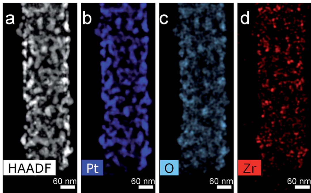
Fig. 6 HAADF STEM image for 4 (a) and EDX mapping for Pt (b), O (c) and Zr (d).
