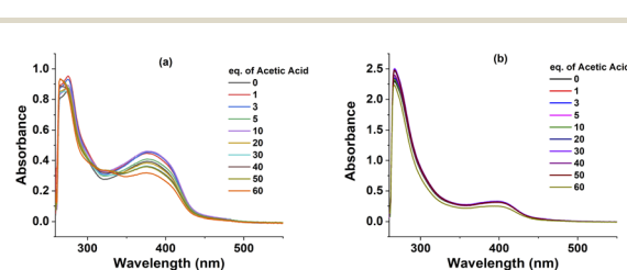
Fig. 4 UV-Vis spectra of complexes 1 (a) and 2 (b) after evaluating electrochemical activity with different concentration of acetic acid.
