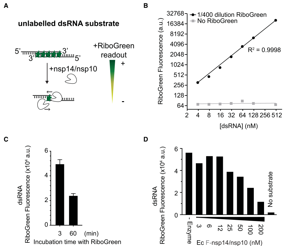
Figure 2. RiboGreen assay for nsp14/nsp10 exonuclease activity.
