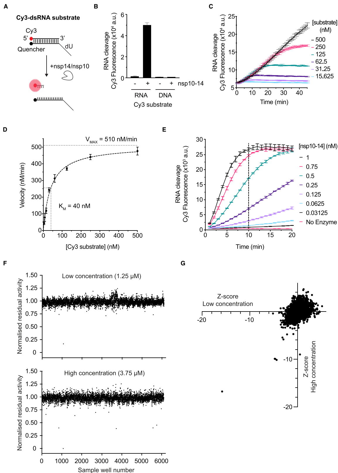
Figure 4. High-throughput screen to identify SARS-CoV-2 nsp14/nsp10 exonuclease inhibitors.
