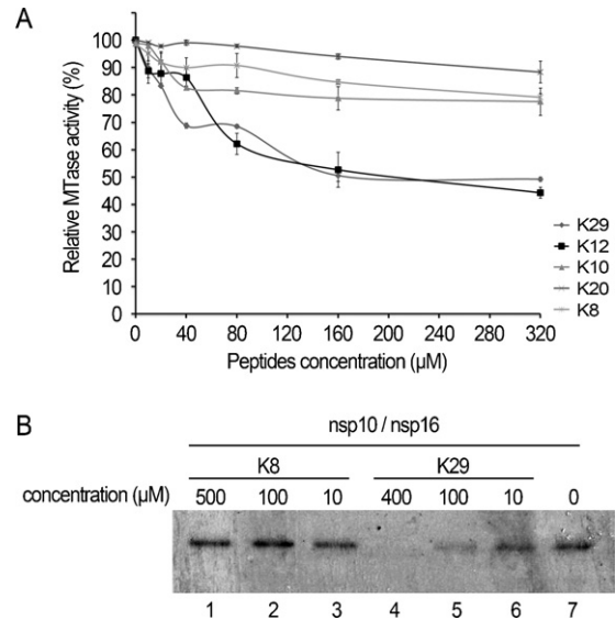
Fig. 4. Inhibitory effect and interference with SAM binding of nsp10/nsp16 complex by short peptides. (A) Inhibition effect of short peptides at different concentrations ( n=3 , mean values \pm SD). (B) SAM binding analyses of SARS-CoV nsp10 and nsp16 at different concentrations of short peptides K8 (lanes 1–3) and K29 (lanes 4–6). The concentrations of the peptides are indicated above the autographic image. The positive control without any peptide added is shown in lane 7.
