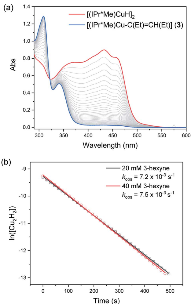
Fig. 8 (a) UV-visible spectra of the reaction of 0.1 mM [(IPr*Me)CuH] 2 with 20 mM 3-hexyne in toluene at 25 °C. (b) First-order fits of kinetics data for reactions of 0.1 mM [(IPr*Me)CuH] 2 with 3-hexyne.
