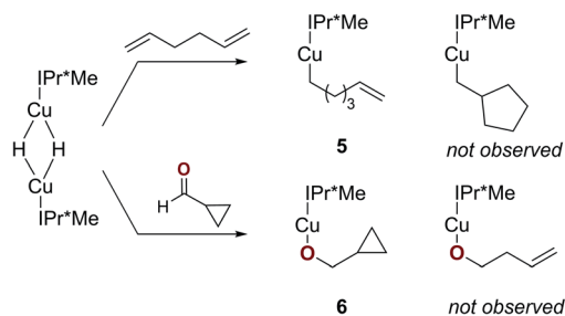
Scheme 3 Reactions of [(IPr*Me)CuH] 2 with radical clock substrates.
