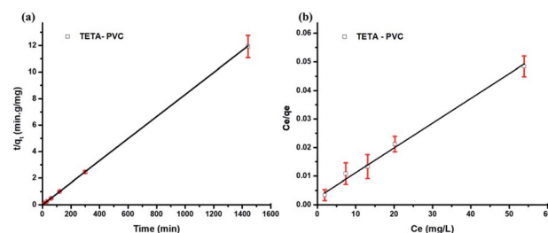
Fig. 6 (a) The pseudo-second-order kinetic plot for the adsorption of ( [Pb(II)] = 150 \text{ mg L}^{-1} ) on a 10 mg TETA-PVC membrane (b) Langmuir isotherm plot for the adsorption of Pb(II) onto TETA-PVC membrane.
