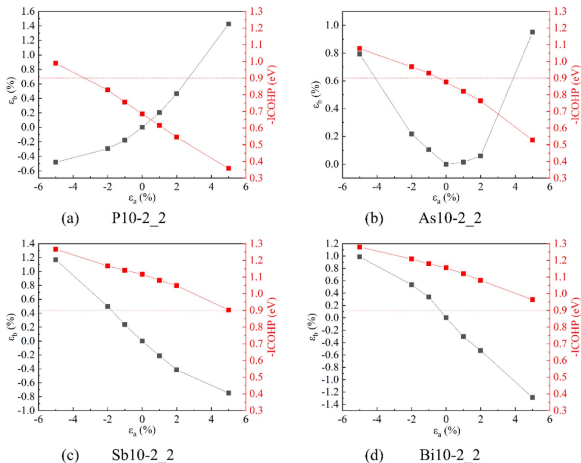
Fig. 11 Mechanical responses of the X10-2_2 phase under strain along the a direction (black lines) and the -ICOHP between X5 and X6 (red lines).
