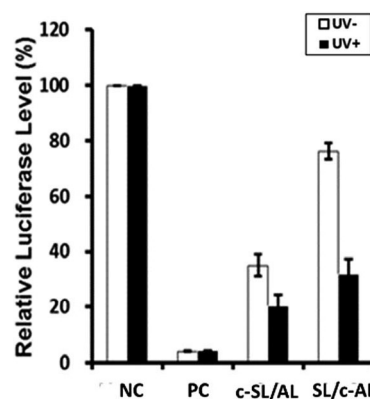
Fig. 4 Photomodulation of firefly luciferase expression in HEK293 cells with caged circular siRNAs using a dual-luciferase assay. "PC", positive control; "c-SL/AL", caged sense stranded siRNA; "SL/c-AL", caged antisense stranded siRNA. The data were averaged in triplicate and all the experiments were repeated three times.
