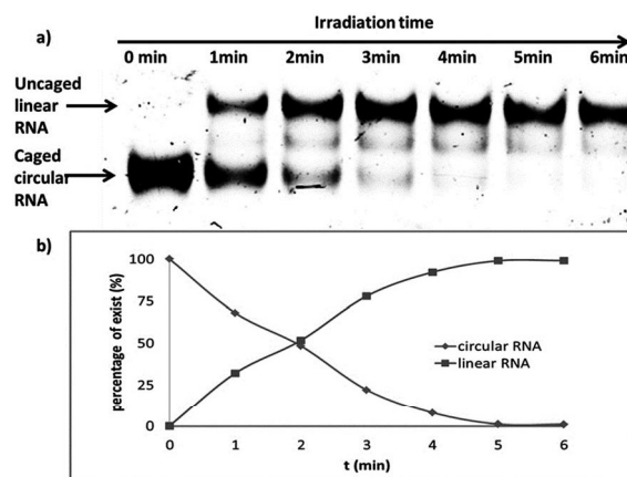
Fig. 2 PAGE (20%) analysis of the photocleavage ability of a caged circular single-stranded RNA (2 \mu M, c-AL) in 1 \times PBS buffer (pH 7.2). The caged RNA was irradiated using a UV-LED lamp (365 nm, 7 mW \text{cm}^{-2} ) for 0, 1, 2, 3, 4, 5 and 6 minutes. The charts are percentages of the circular and cleaved RNAs upon light irradiation at different time intervals after gel was quantified with ImageQuant.
