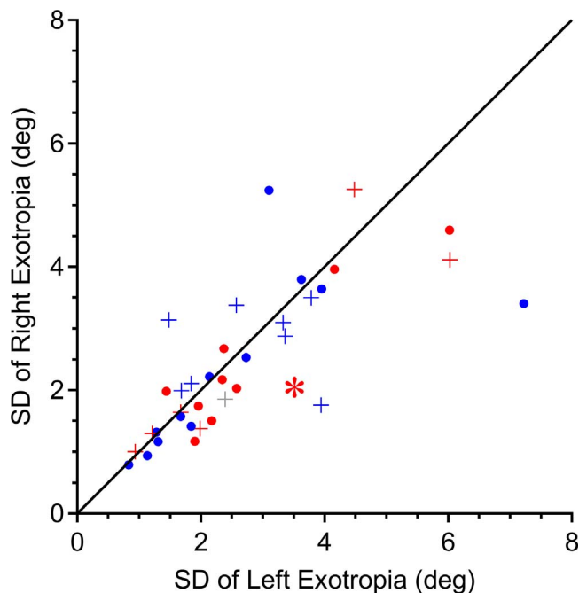
FIGURE 6. Eye preference is not correlated with variability of deviation angle. The standard deviation of exotropia is plotted for the right eye fixating and for the left eye fixating for each subject. The standard deviations are correlated ( r = 0.74 ), but there is no clear relationship with eye dominance (red = right eye dominant, blue = left eye dominant). If fixation by the dominant eye rendered the exotropia more stable, blue points would be located above the line and red points below. +, subjects with > 2^\circ incomitance. *Patient illustrated in Figure 2.
