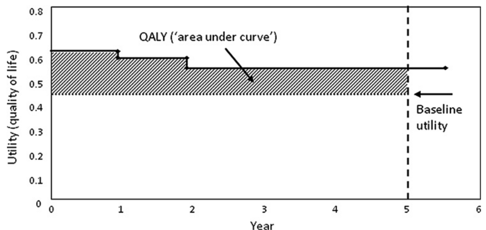
Figure 1 Schematic calculation of quality-adjusted life years (QALYs).
