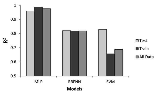
Fig. 8 The performance measures of the designed PDNFMs.
