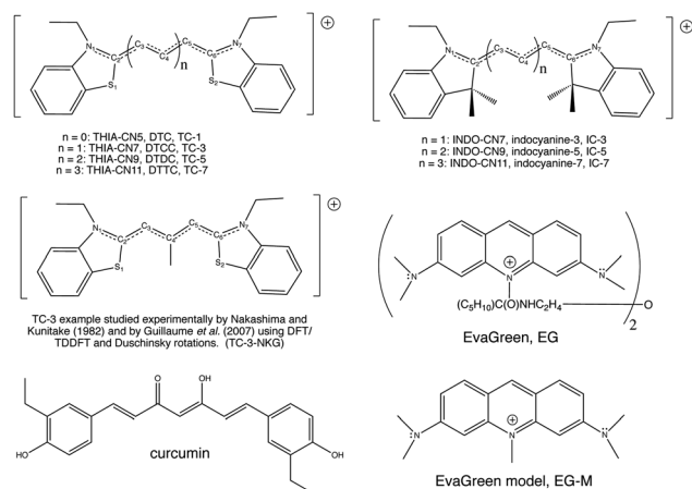
Fig. 2 Molecular structures of 3,3'-diethylthiacarbocyanine, 3,3'-diethylthiadibenzocarbocyanine, 3,3'-diethylthiatriazabenzocarbocyanine (top left), TC-3-NKG example (middle left), curcumin (bottom left), 1,1'-diethyl-3,3,3',3'-tetramethylindocarbocyanine, 1,1'-diethyl-3,3,3',3'-tetramethylindodicarbocyanine, 1,1'-diethyl-3,3,3',3'-tetramethylindotricarbocyanine (top right), EvaGreen (middle right), a model of the EvaGreen fluorophore (bottom right). Common abbreviations are included. Hydrogen atoms bonded to the polymethine chain carbon atoms are not shown. Atom numbering shown here will be referred to in the text.
