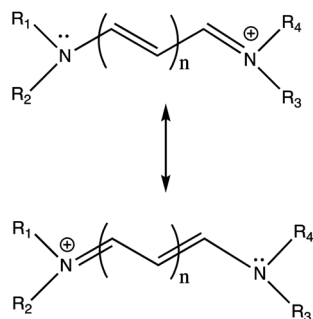
Fig. 1 Prototypical cyanine dye resonance structures.
