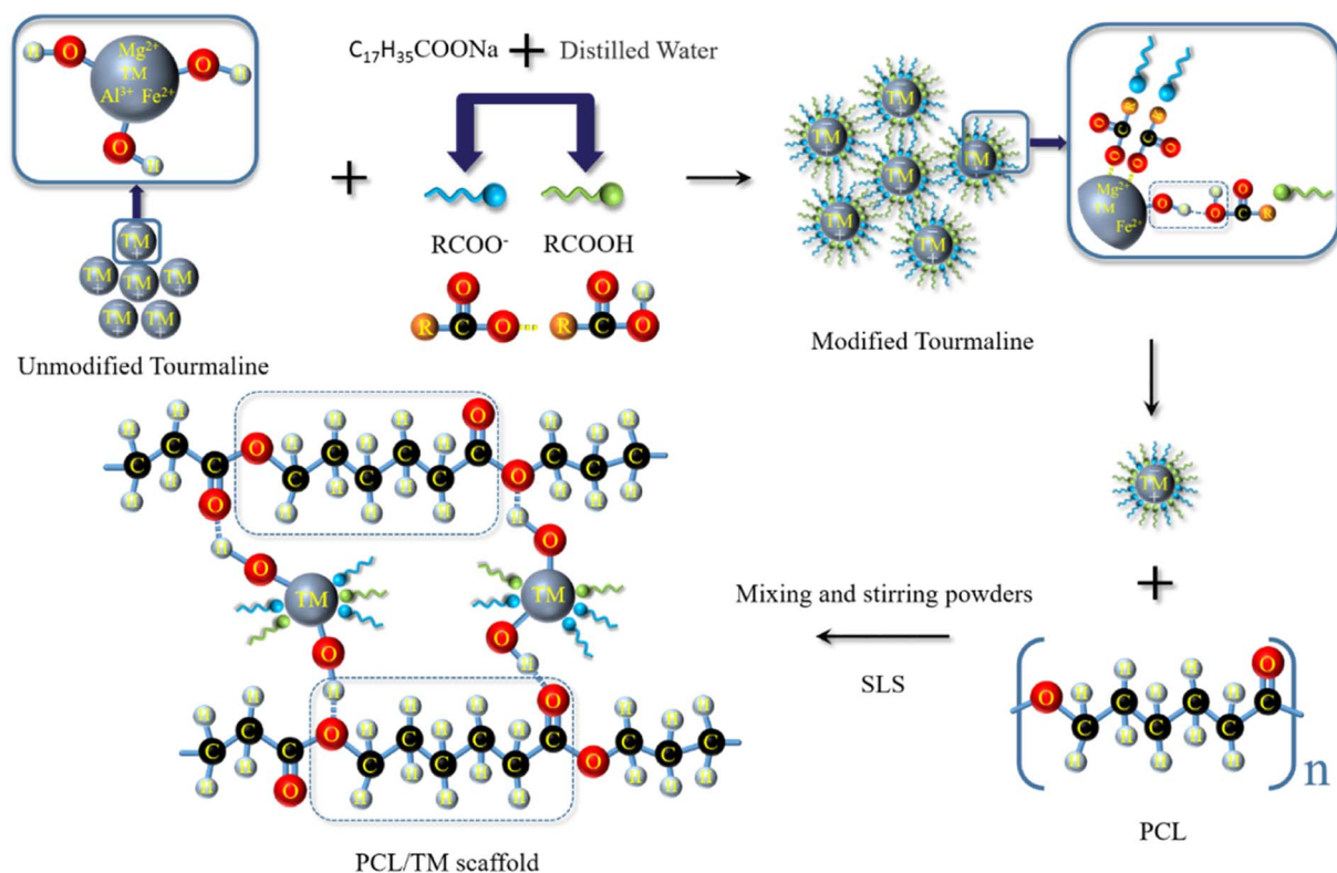
Fig. 9 Mechanism of action of sodium stearate on TM modification.
